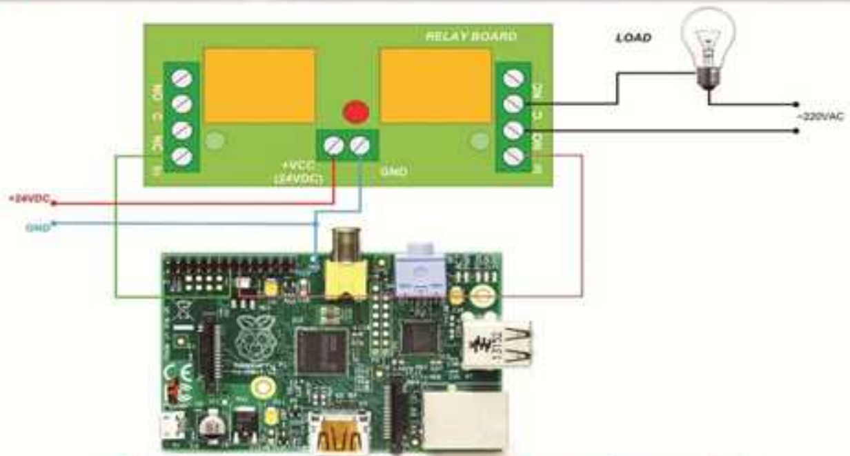
Connection of Relay to Raspberry Pi
